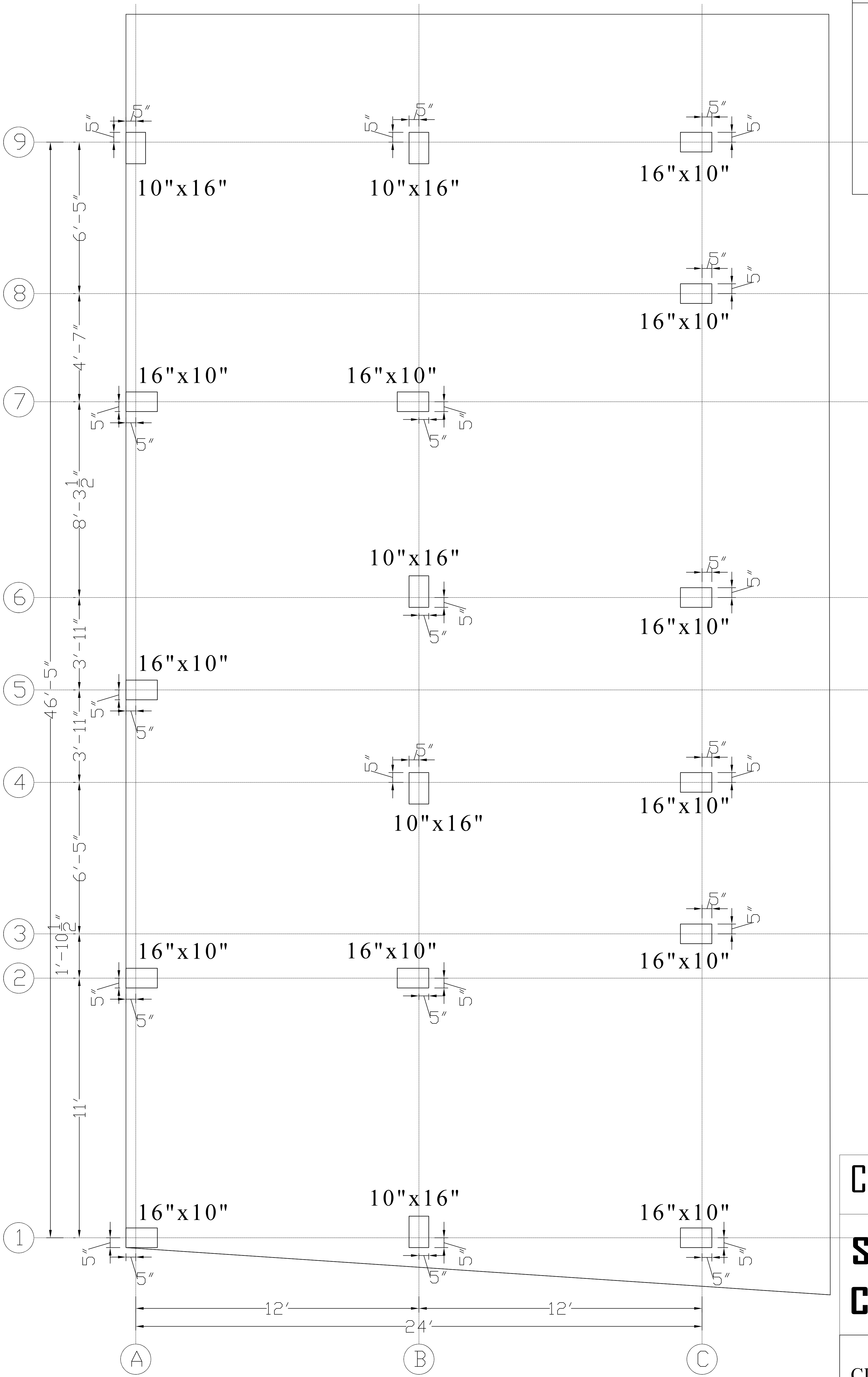
FOUNDATION LAYOUT PLAN
